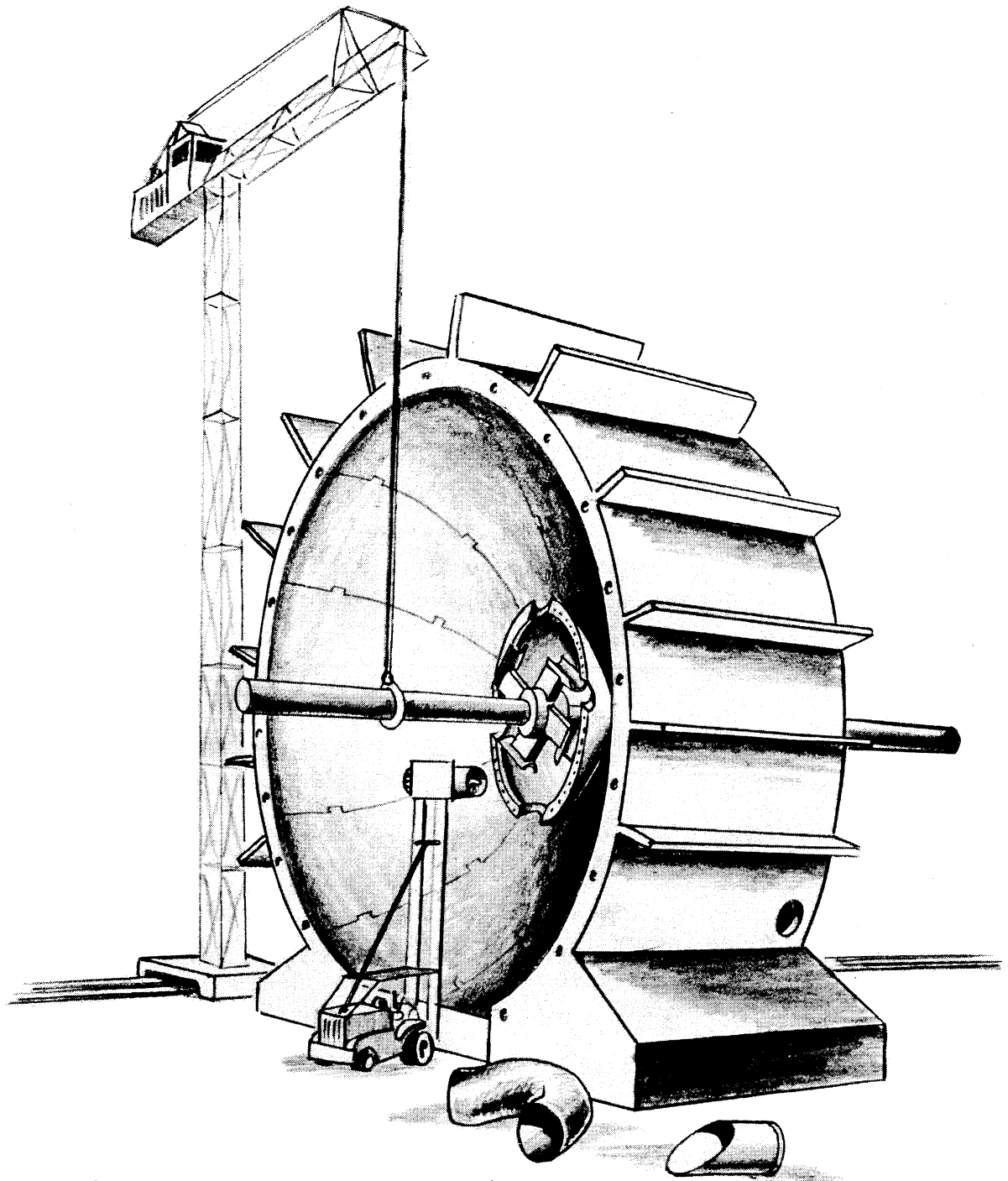
Exhibit 3. Install shaft, Front side of Aerodynamic Shell and Engine mounts.
